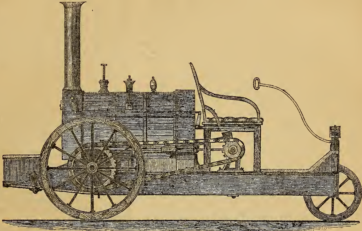
LOCOMOTIVE STEAM CARRIAGE FOR COMMON ROADS.
